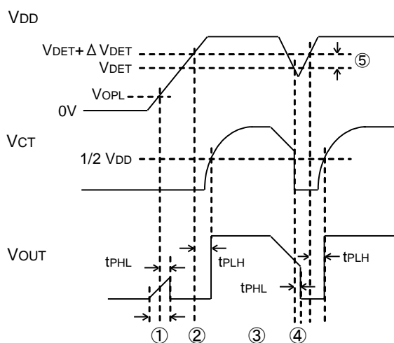
Fig.17 Timing Waveform
