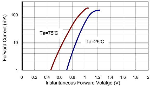
FIG 1 Typical Forward Characteristics
