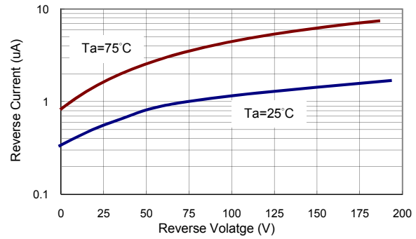
FIG 2 Reverse Current vs Reverse Voltage
