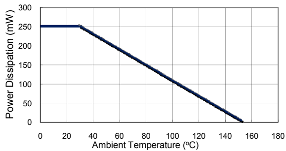
FIG 3 Admissible Power Dissipation Curve
