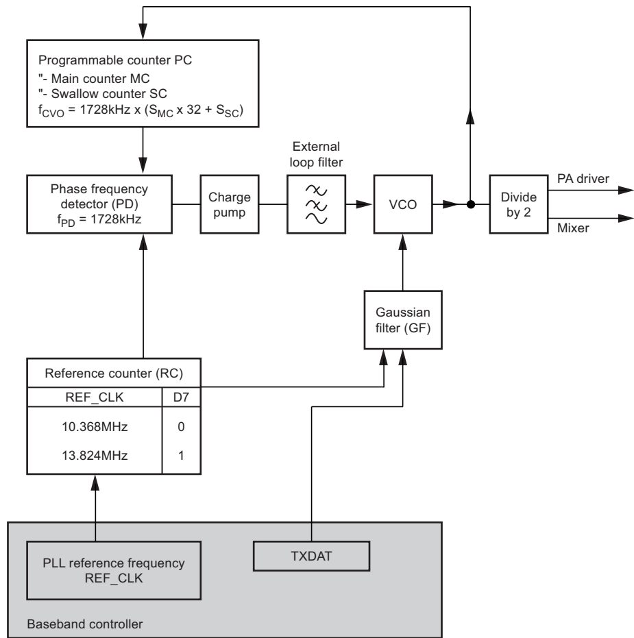
Figure 8-1. PLL Principle
