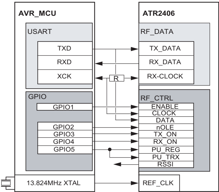
Figure 9-2. Example with AVR MCU
