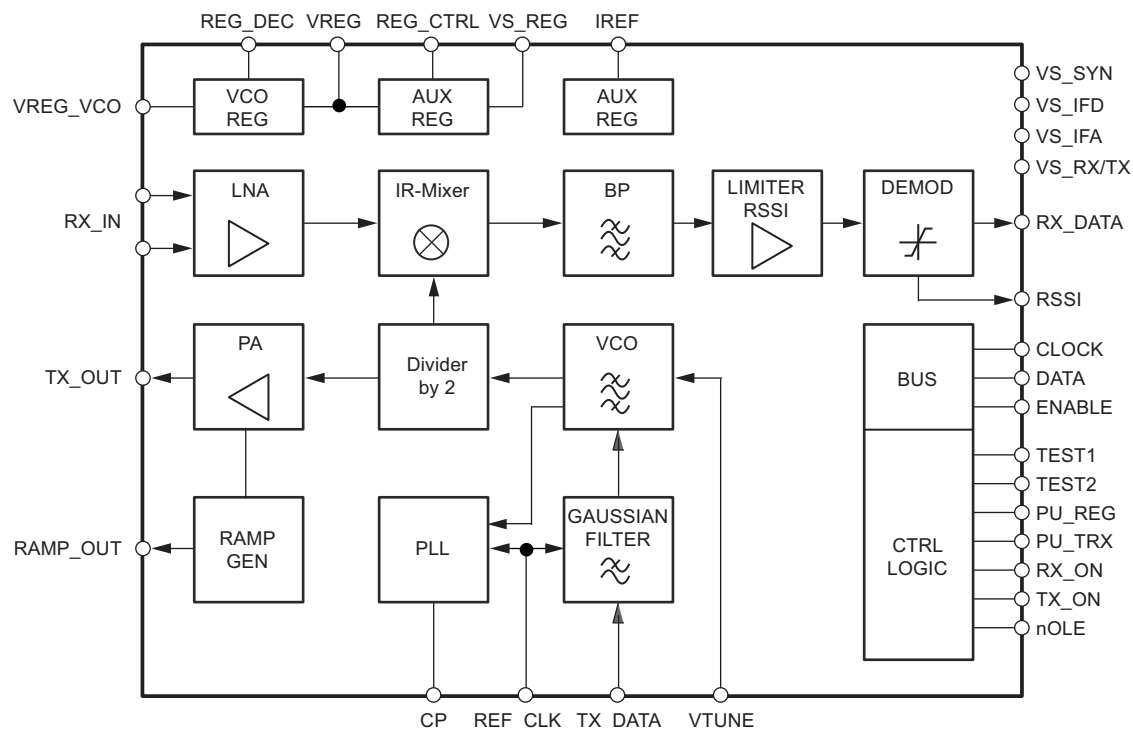
Figure 1-1. Block Diagram
