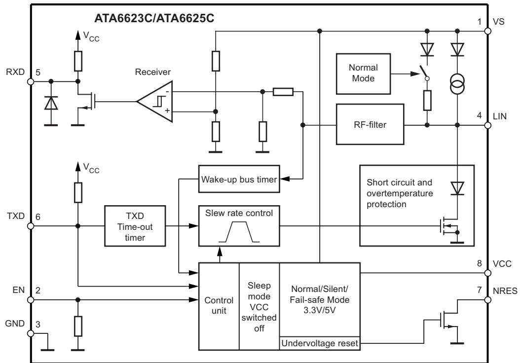
Figure 1-1. Block Diagram
