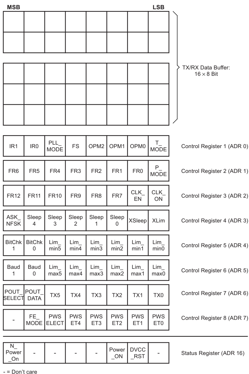
Figure 9-1. Register Structure
