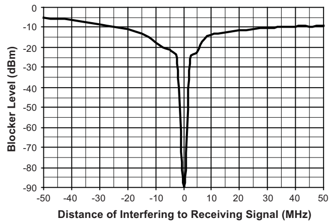
Figure 5-7. \pm 50\text{MHz} Blocking Characteristic for -85\text{dBm} Useful Signal at 433.92\text{MHz}
