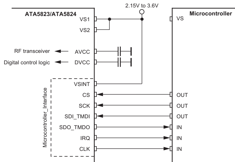
Figure 7-5. Battery Application
