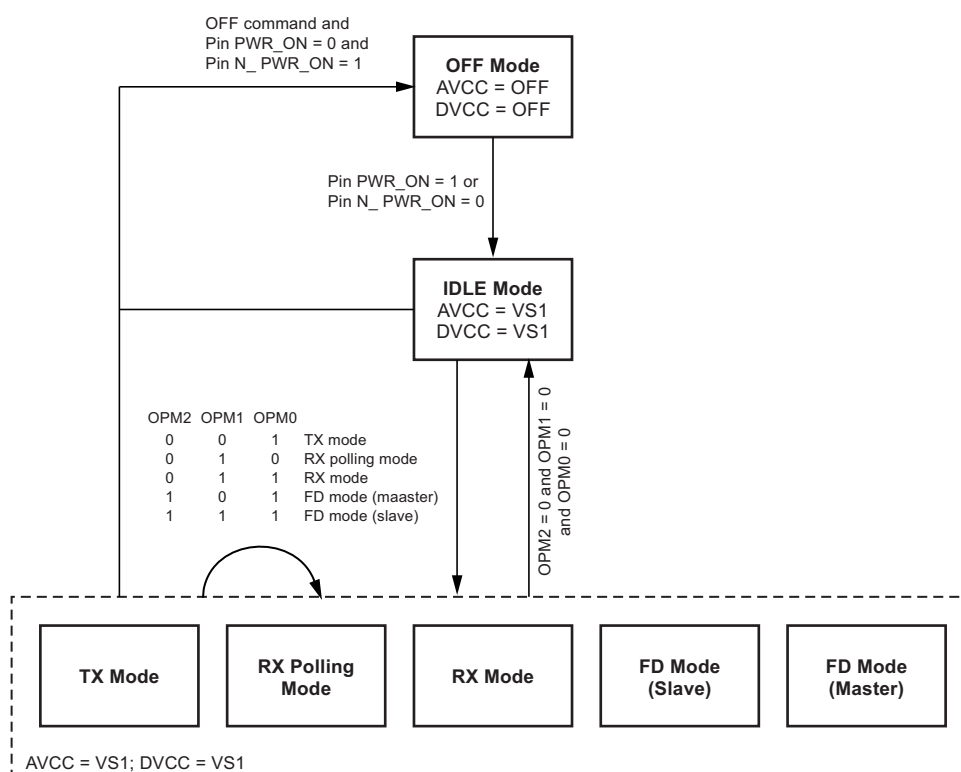
Figure 7-2. Flow Chart Operation Modes
