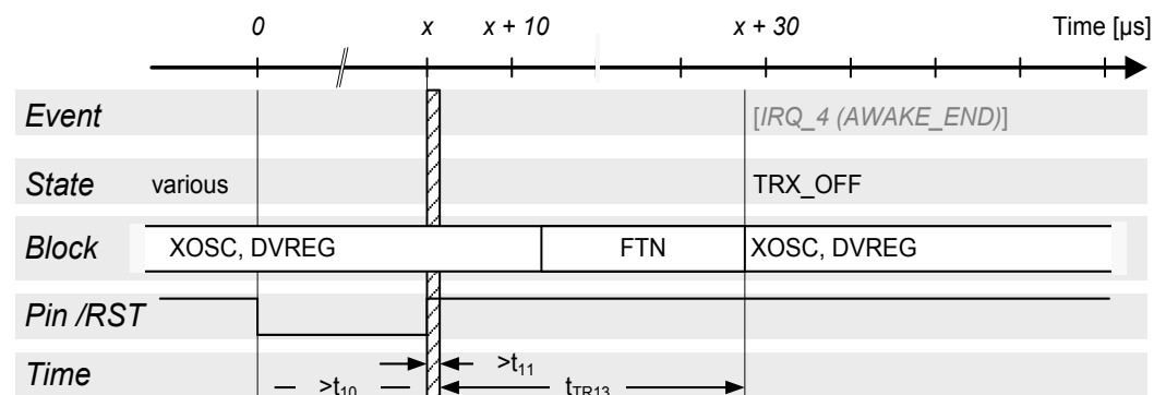
Figure 7-8. Reset Procedure.
