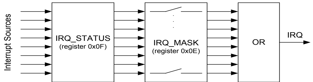
Figure 6-22. IRQ_MASK_MODE = 1.
