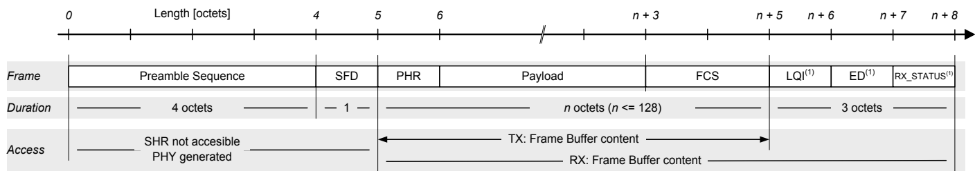
Figure 9-8. AT86RF233 Frame Structure.
