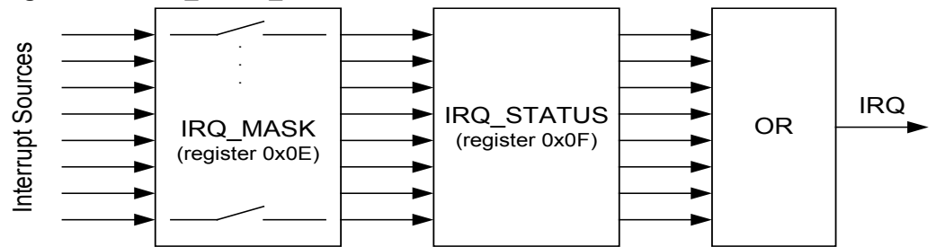
Figure 6-21. IRQ_MASK_MODE = 0.
