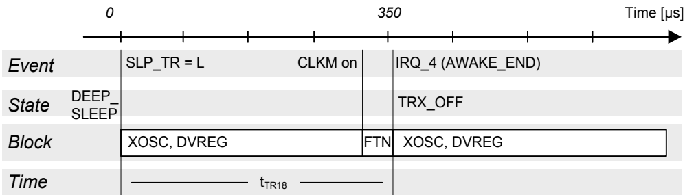
Figure 7-5. Wake-up Procedure from DEEP_SLEEP State.
