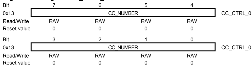
Figure 9-19. Register CC_CTRL_0.
