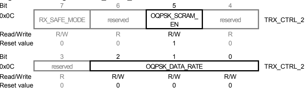
Figure 11-13. Register TRX_CTRL_2.
