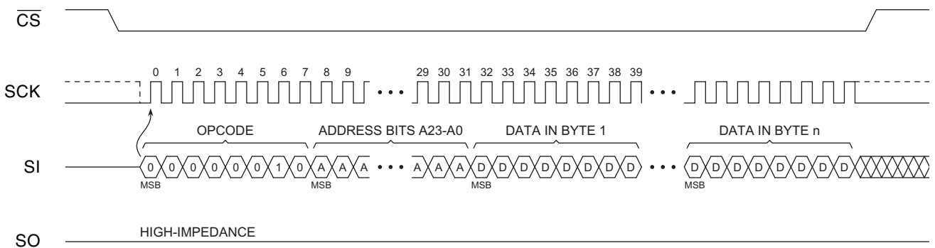
Figure 8-2. Page Program
