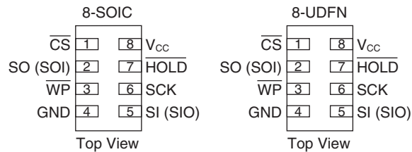
Figure 2-1. Pin Configurations
