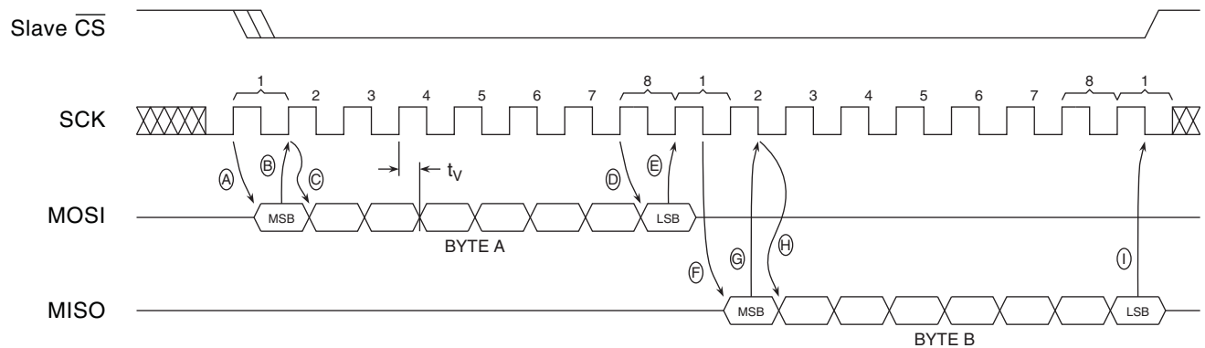
Figure 13-1. RapidS Operation
