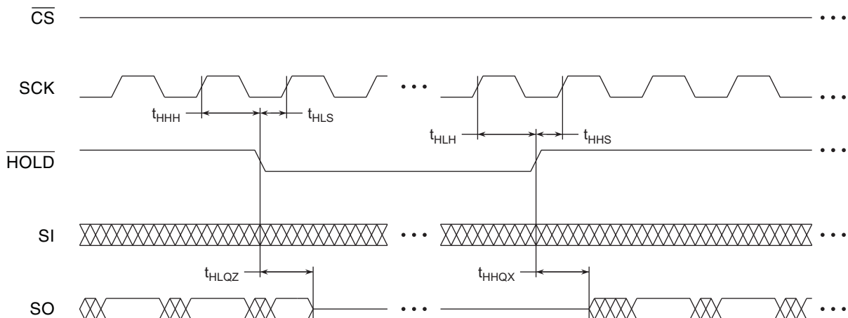
Figure 16-5. \overline{HOLD} Timing – Serial Output
