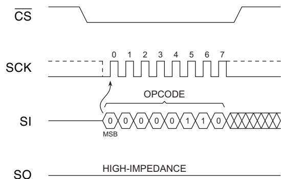
Figure 9-1. Write Enable
