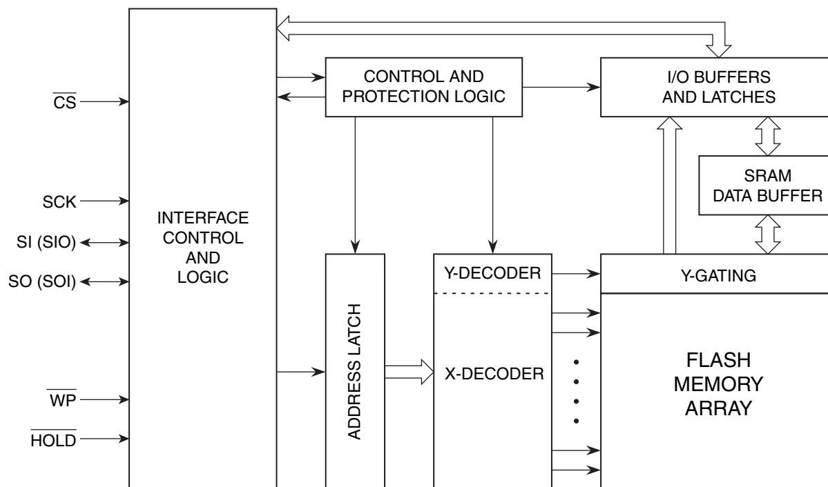
Figure 3-1. Block Diagram
