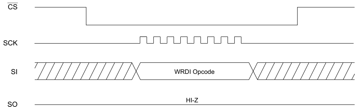
Figure 7-3. WRDI Timing
