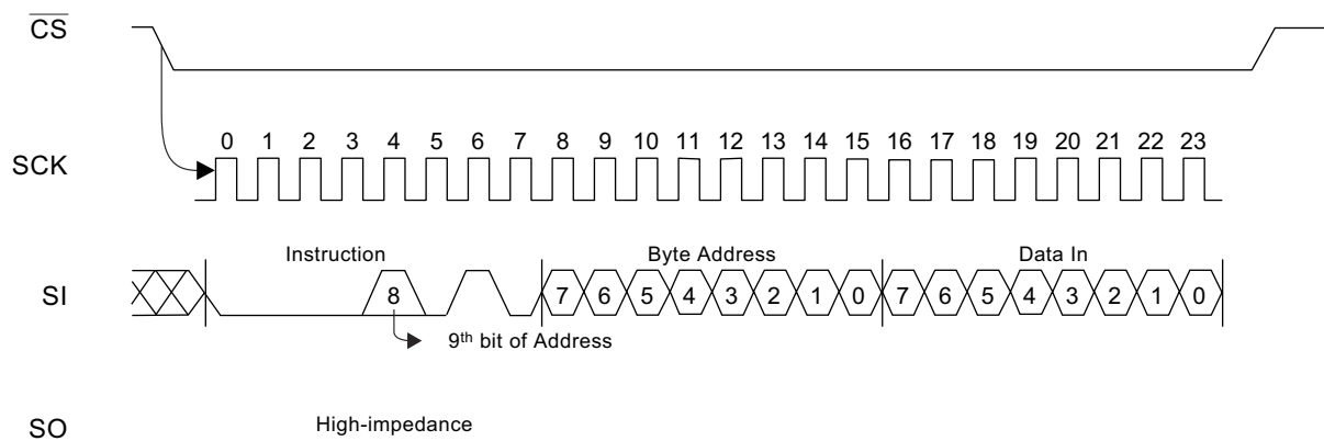
Figure 7-7. WRITE Timing
