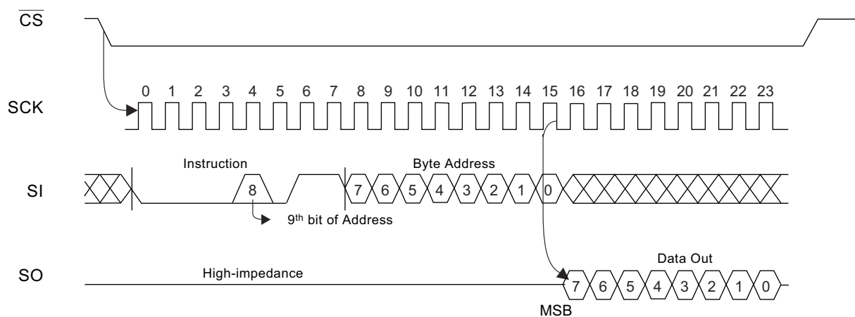
Figure 7-6. READ Timing
