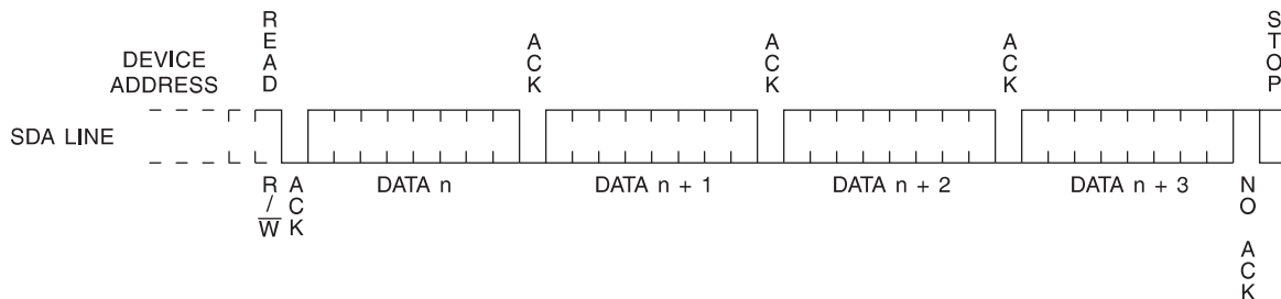
Figure 6-6. Sequential Read
