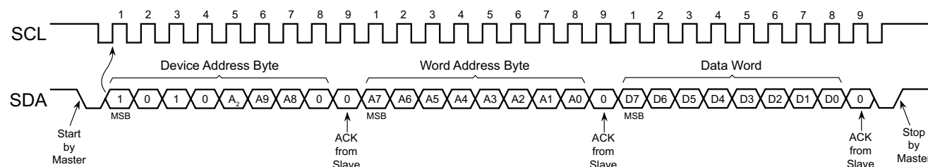
Figure 5-1. Byte Write
