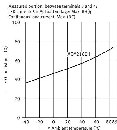
2-3. On resistance vs. ambient temperature characteristics
