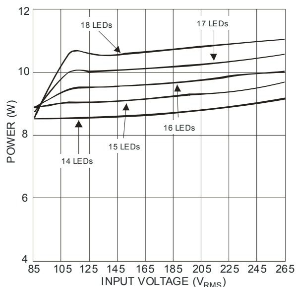
180mA LED Driver Input Power Dissipation vs. Input Voltage
