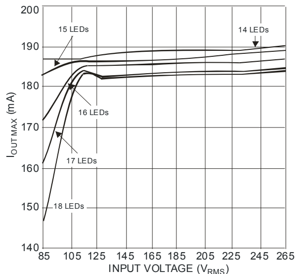
180mA LED Driver Output Current vs. Input Voltage
