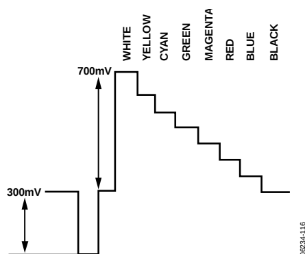
Figure 118. Y Levels—NTSC
