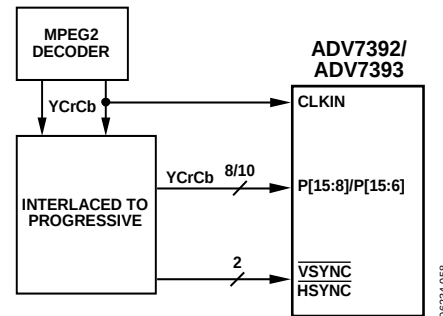
Figure 60. ED/HD-DDR Example Application
