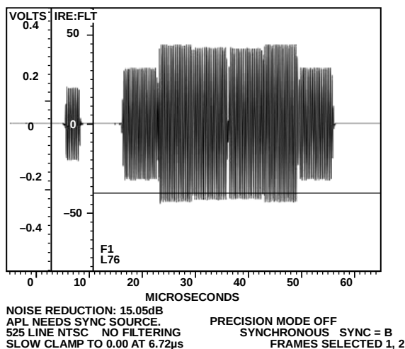
Figure 134. NTSC Chroma
