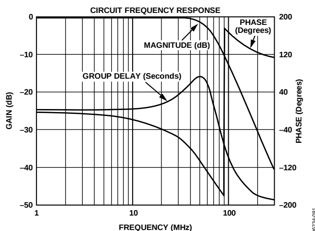
Figure 92. Output Filter Plot for HD, 4× Oversampling
