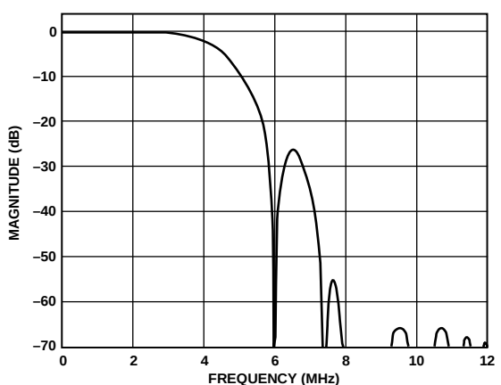
Figure 29. SD NTSC, Luma Low-Pass Filter Response
