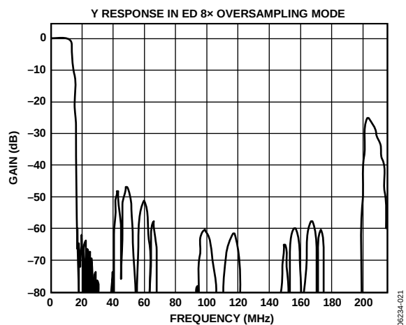
Figure 23. ED 8x Oversampling, Y Filter Response
