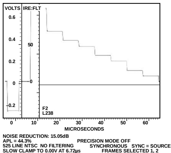
Figure 133. NTSC Luma
