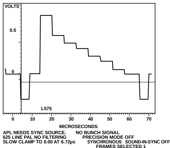
Figure 136. PAL Luma
