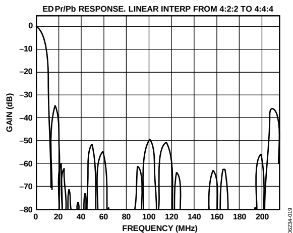
Figure 21. ED 8x Oversampling, Pr/Pb Filter (Linear) Response
