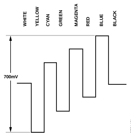
Figure 123. Pb Levels—PAL
