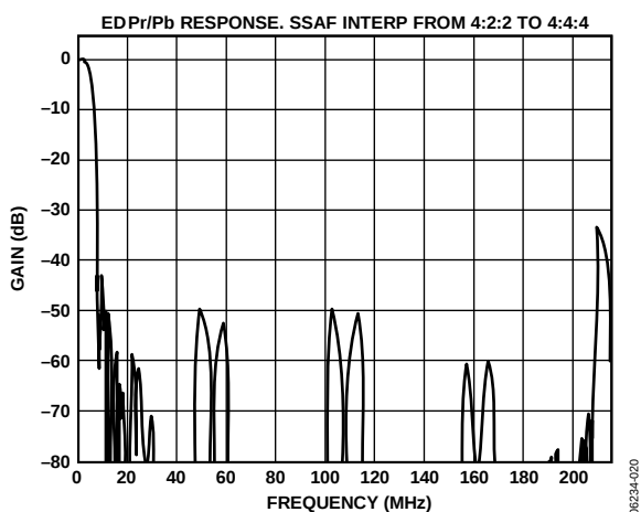
Figure 22. ED 8x Oversampling, Pr/Pb Filter (SSAF™) Response
