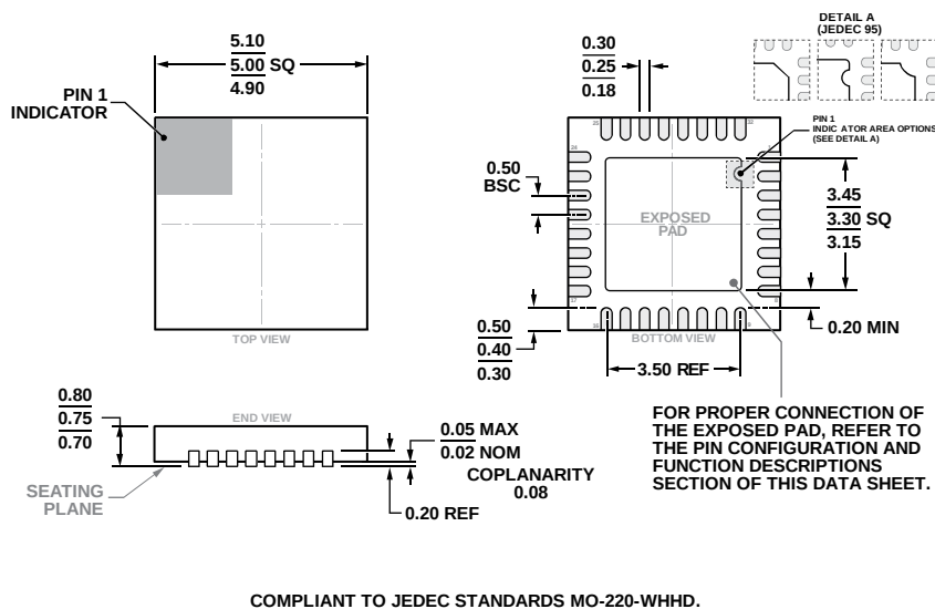
Figure 146. 32-Lead Lead Frame Chip Scale Package [LFCSP] 5 mm x 5 mm Body and 0.75 mm Package Height (CP-32-13)
