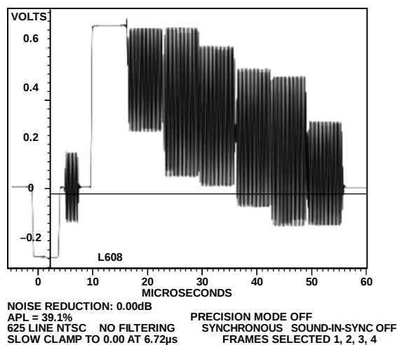
Figure 135. PAL Color Bars (75%)
