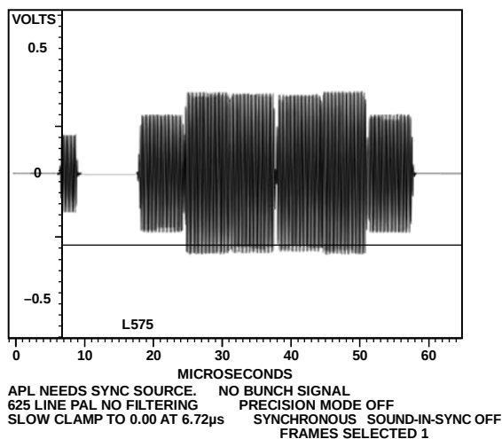
Figure 137. PAL Chroma
