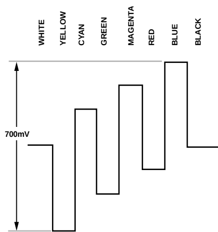
Figure 120. Pb Levels—NTSC
