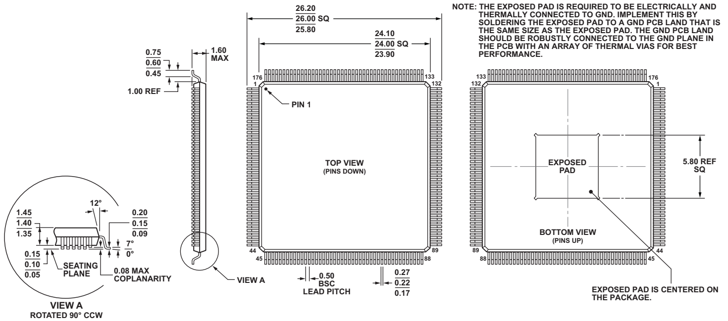
Figure 71. 176-Lead Low Profile Quad Flat Package [LQFP_EP] (SQ-176-2) Dimensions shown in millimeters
