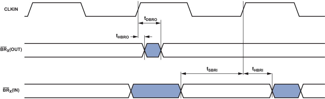
Figure 21. Shared Memory Bus Request
