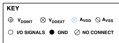
Figure 49. 256-Ball BGA_ED Ball Configuration (Top View)
