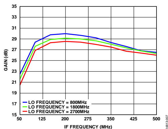
Figure 7. Gain vs. IF Frequency; RF Sweep with Fixed LO, L_{SHUNT} = 150\text{ nH}
