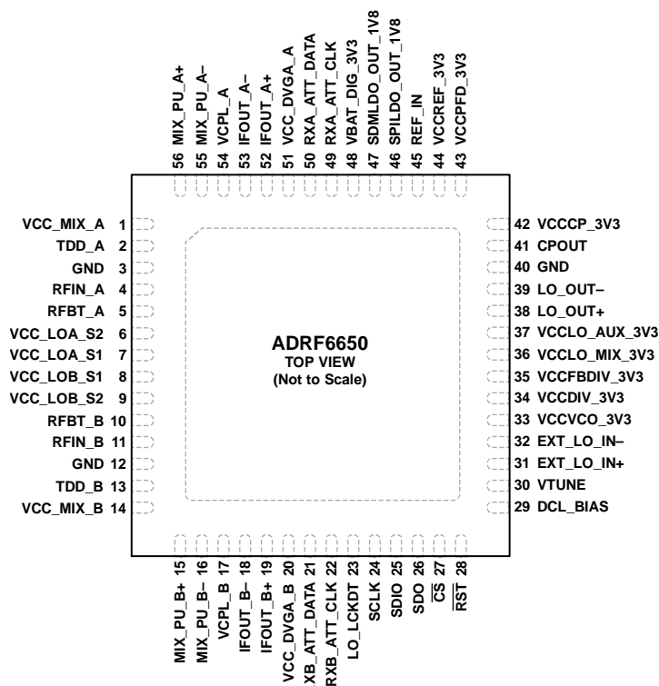
Figure 3. Pin Configuration
