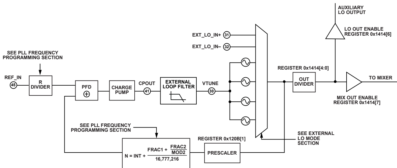
Figure 52. PLL/VCO Block Diagram
