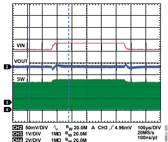
Figure 25. Buck Response to Line Transient, V IN = 4.5 V to 5.0 V, VOUT1 = 1.8 V, PWM Mode
