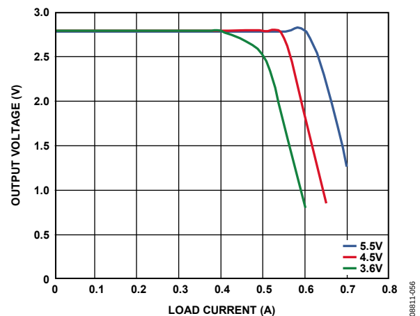
Figure 44. LDO1, LDO2 Output Current Capability vs. Input Voltage
