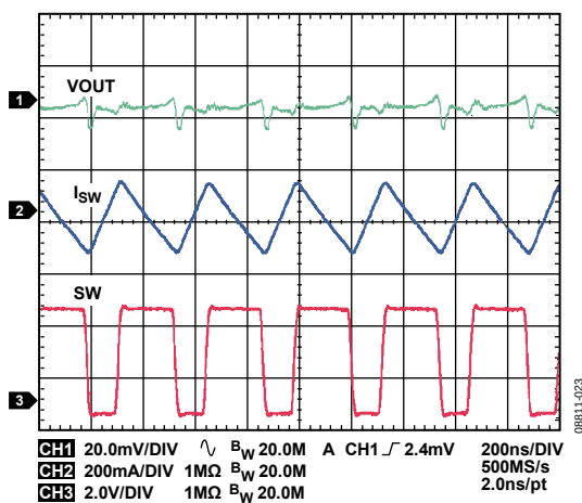
Figure 23. Typical Waveforms, VOUT1 = 3.3 V, IOUT2 = 30 mA, PWM Mode
