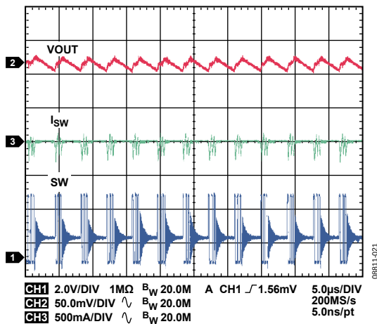
Figure 21. Typical Waveforms, VOUT1 = 1.8 V, IOUT2 = 30 mA, Auto Mode
