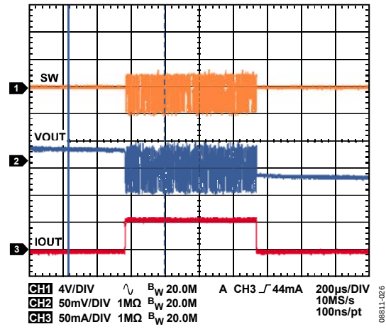
Figure 26. Buck Response to Load Transient, IOUT1 from 1 mA to 50 mA, VOUT1 = 3.3 V, Auto Mode
