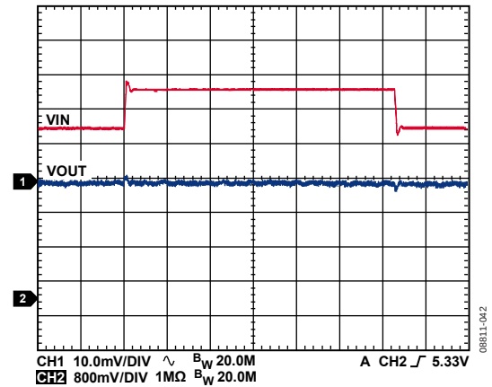
Figure 42. LDO2 Response to Line Transient, Input Voltage from 4.5 V to 5.5 V, V_{OUT3} = 3.3\text{ V}
