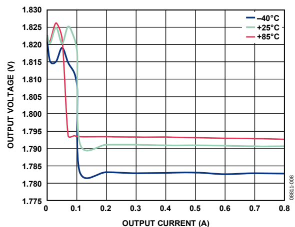
Figure 8. Buck Load Regulation Across Temperature, VOUT1 = 1.8 V, Auto Mode
