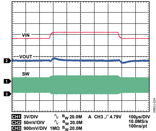
Figure 24. Buck Response to Line Transient, Input Voltage from 4.5 V to 5.0 V, VOUT1 = 3.3 V, PWM Mode
