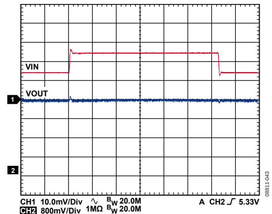
Figure 43. LDO1 Line Transient V_{IN} = 4.5\text{ V} to 5.5\text{ V} , V_{OUT2} = 1.5\text{ V}
