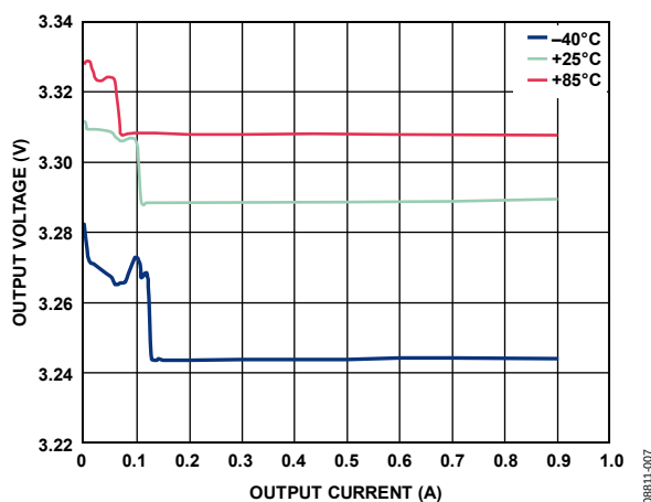
Figure 7. Buck Load Regulation Across Temperature, VOUT1 = 3.3 V, Auto Mode
