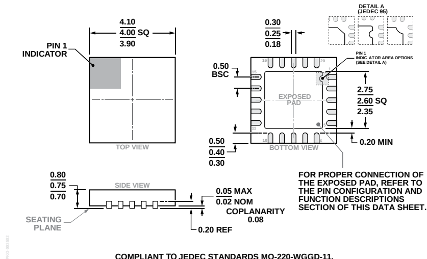
Figure 70. 20-Lead, Lead Frame Chip Scale Package [LFCSP] 4 mm × 4 mm Body and 0.75 mm Package Height (CP-20-8) Dimensions shown in millimeters
