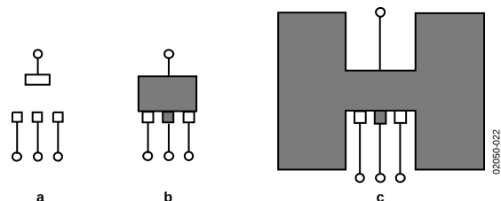
Figure 22. PCB Layouts
