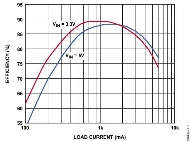
Figure 7. Efficiency, Combined Dual-Phase Output, V_{OUT} = 1.2V and f_{SW} = 1.2 MHz ; Inductor TOKO FDV0620-1R0M, 1.0 \mu H , 14 m\Omega
