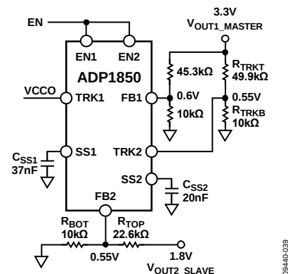
Figure 39. Example of a Ratiometric Tracking Circuit
