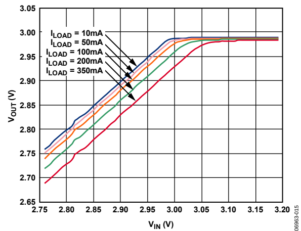
Figure 15. Output Voltage vs. Input Voltage (in Dropout), V_{OUT} = 3\text{ V}
