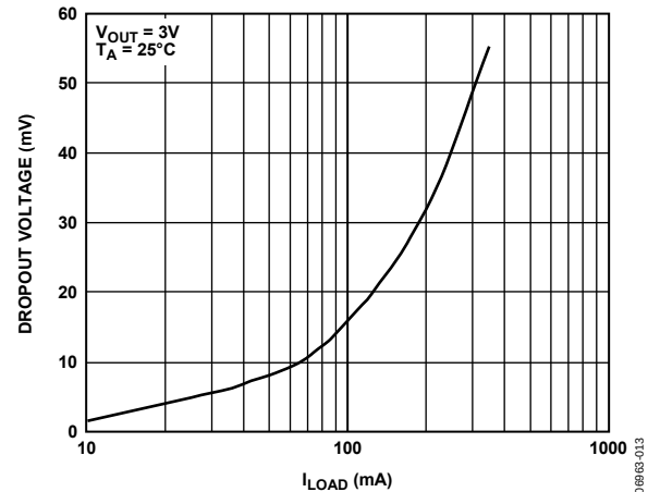
Figure 13. Dropout Voltage vs. Load Current, V_{OUT} = 3\text{ V}
