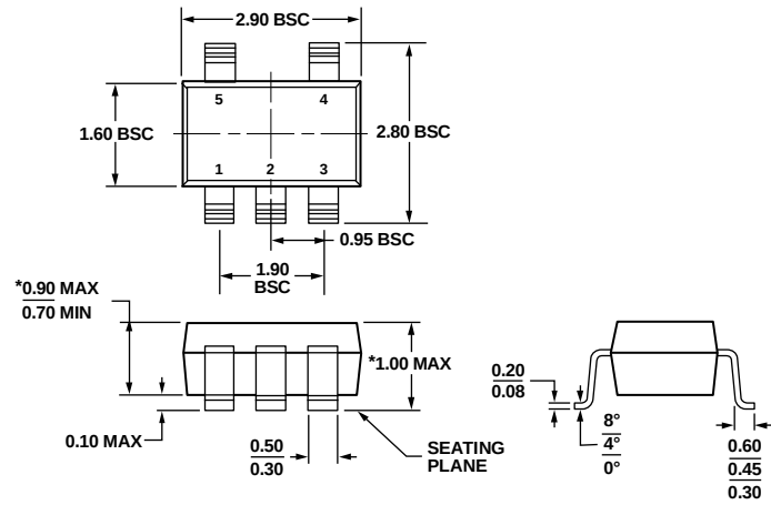
*COMPLIANT TO JEDEC STANDARDS MO-193-AB WITH THE EXCEPTION OF PACKAGE HEIGHT AND THICKNESS. Figure 48. 5-Lead Thin Small Outline Transistor Package [TSOT] (UJ-5) Dimensions show in millimeters
