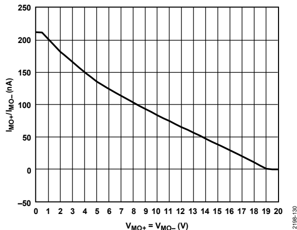
Figure 40. I_{MO+}/I_{MO-} vs. V_{MO+}/V_{MO-} with V_{CC} = 20\text{ V}
