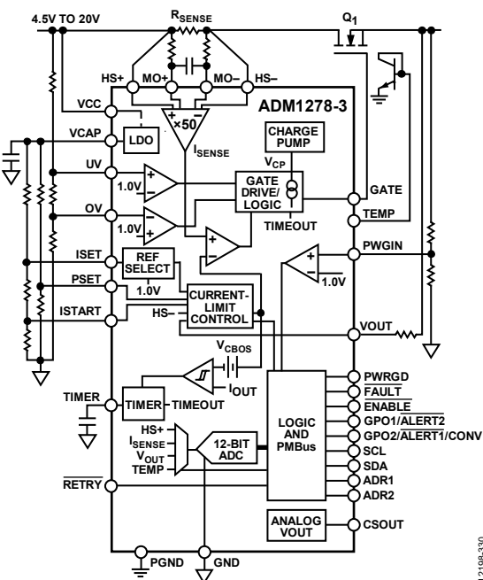
Figure 73. ADM1278-3 Typical Application Circuit
