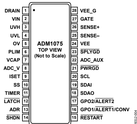
Figure 3. TSSOP Pin Configuration
