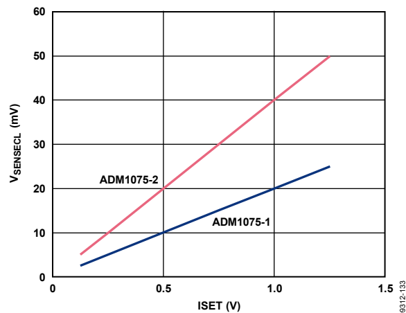
Figure 34. Typical Hot Swap V_{SENSECL} vs. ISET
