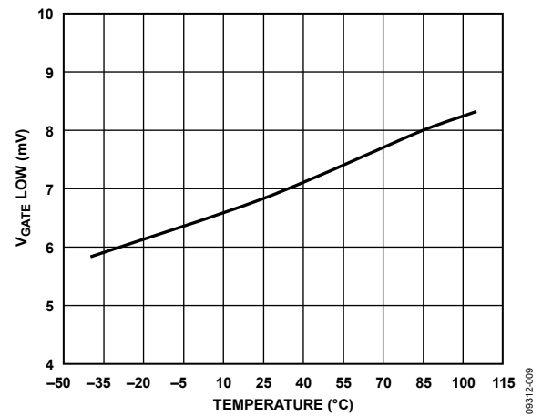
Figure 9. V_{GATE\ Low} vs. Temperature ( I_{GATE} = 100\text{ }\mu\text{A} )
