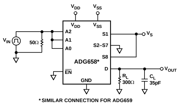
Figure 26. Break-Before-Make Delay, t_{\text{BBM}}
