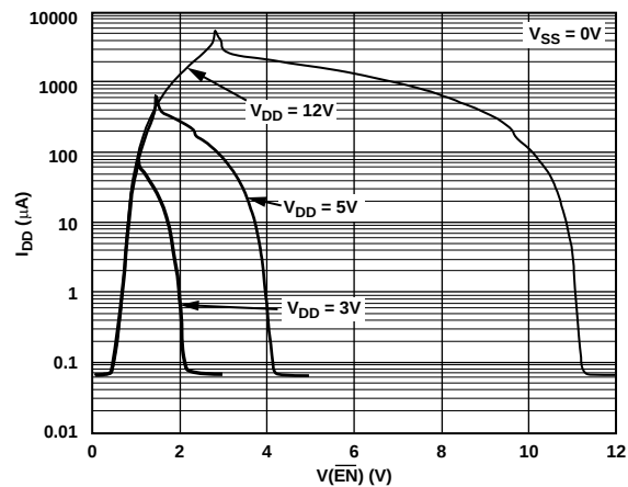
Figure 19. V_{DD} Current vs. Logic Level
