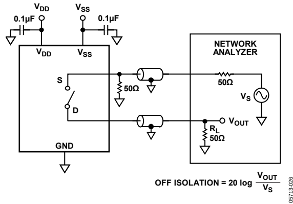
Figure 38. Off Isolation
