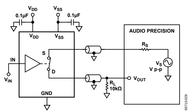
Figure 41. THD + N
