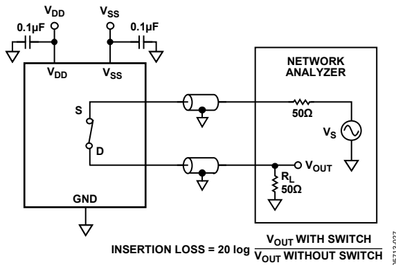
Figure 39. Bandwidth
