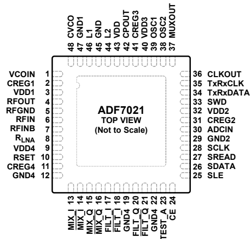
Figure 10. Pin Configuration
