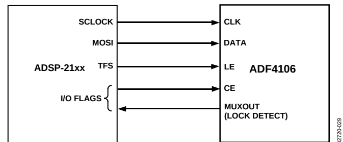
Figure 24. ADSP-21xx-to-ADF4106 Interface
