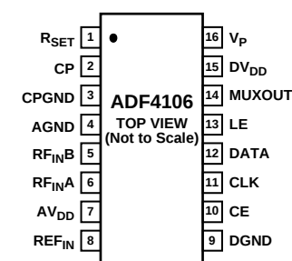
Figure 3. 16-Lead TSSOP Pin Configuration
