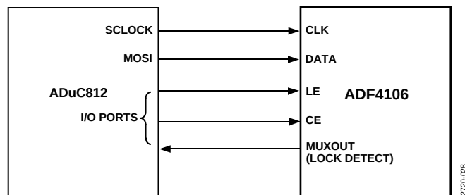
Figure 23. ADuC812-to-ADF4106 Interface
