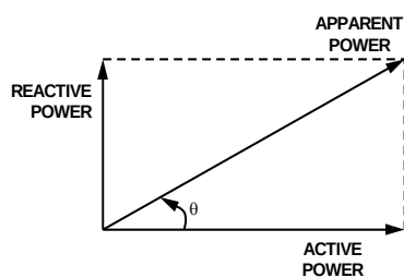
Figure 72. Power Triangle
