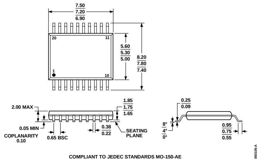
COMPLIANT TO JEDEC STANDARDS MO-150-AE Figure 98. 20-Lead Shrink Small Outline Package [SSOP] (RS-20) Dimensions shown in millimeters
