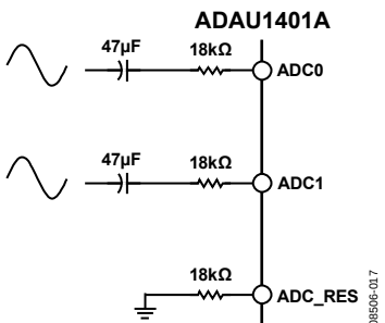
Figure 17. Audio ADC Input Configuration
