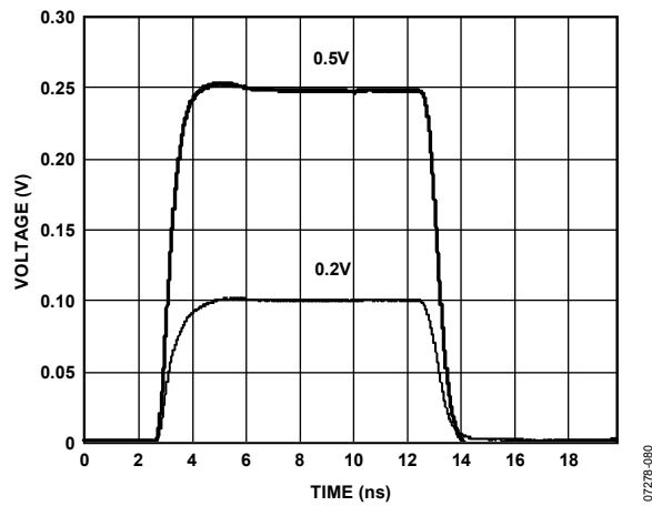
Figure 4. Driver Small Signal Response; V_H = 0.2\text{ V}, 0.5\text{ V}; V_L = 0.0\text{ V}; 50\ \Omega Termination
