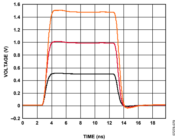
Figure 5. Driver Large Signal Response; V_H = 1.0\text{ V}, 2.0\text{ V}, 3.0\text{ V}; V_L = 0.0\text{ V}; 50\ \Omega Termination
