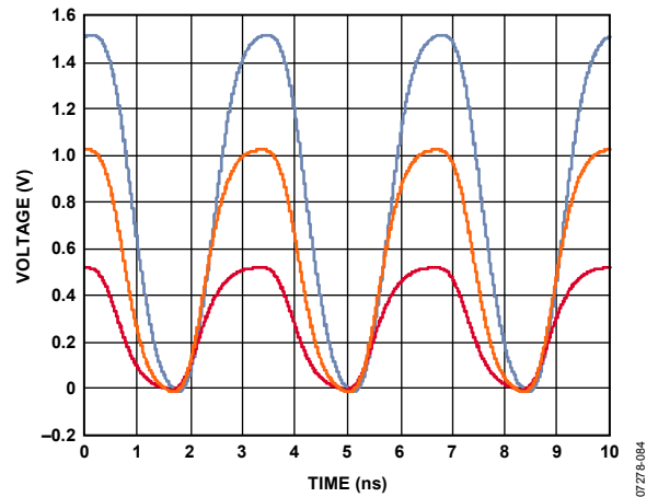
Figure 8. 300 MHz Driver Response; V_H = 1.0\text{ V}, 2.0\text{ V}, 3.0\text{ V}; V_L = 0.0\text{ V}; 50\ \Omega Termination
