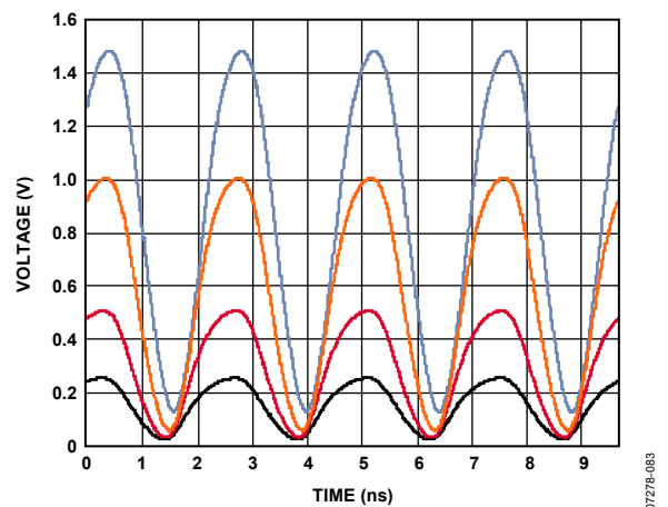
Figure 9. 400 MHz Driver Response; V_H = 0.5\text{ V}, 1.0\text{ V}, 2.0\text{ V}, 3.0\text{ V}; V_L = 0.0\text{ V}; 50\ \Omega Termination
