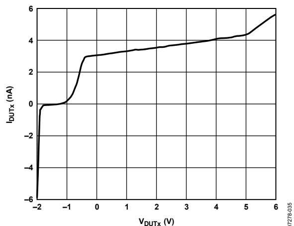
Figure 46. DUTx Pin Leakage Current in High-Z Mode
