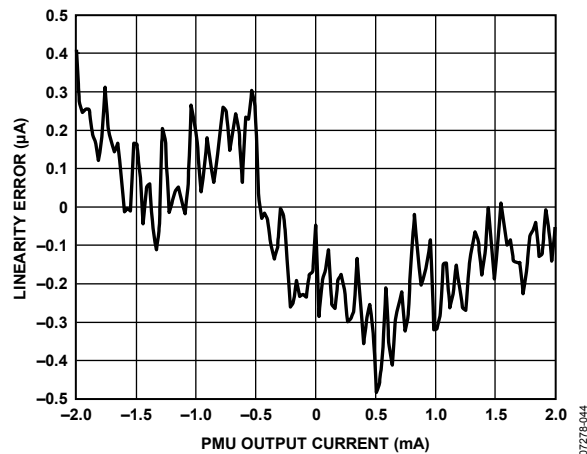
Figure 50. PMU Force Current Range B Linearity
