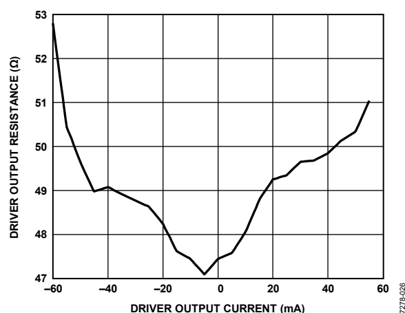
Figure 26. Driver Output Resistance vs. Output Current
