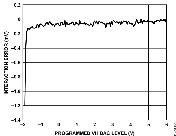
Figure 25. Driver Interaction Error; VL = -2.0 V; VH Swept from -1.9 V to +6.0 V
