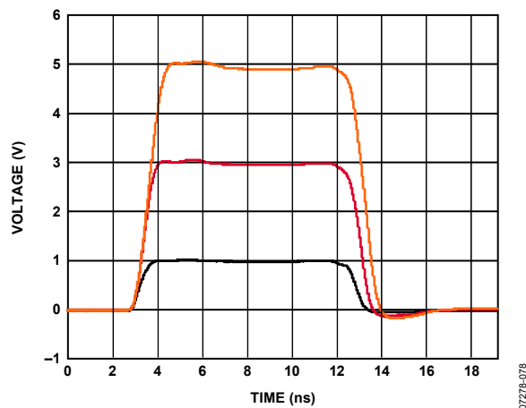
Figure 6. Driver Large Signal Response; V_H = 1.0\text{ V}, 3.0\text{ V}, 5.0\text{ V}; V_L = 0.0\text{ V}; 500\ \Omega Termination
