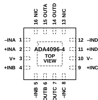
Figure 7. 16-Lead LFCSP (CP-16-22), ADA4096-4
