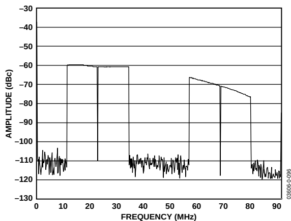
Figure 66. AD9861 Tx Path FFT of OFDM Signal in Figure 52 with 1 \times Interpolation
