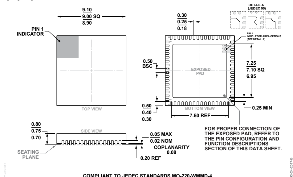
Figure 87. 64-Lead Lead Frame Chip Scale Package [LFCSP] 9 mm x 9 mm Body and 0.75 mm Package Height (CP-64-12)
