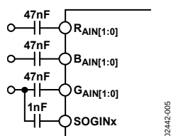
Figure 6. Typical Clamp Configuration for RGB/YUV Applications
