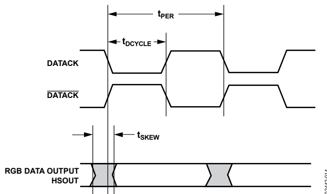
Figure 15. Output Timing
