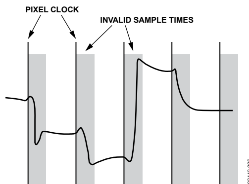
Figure 7. Pixel Sampling Times
