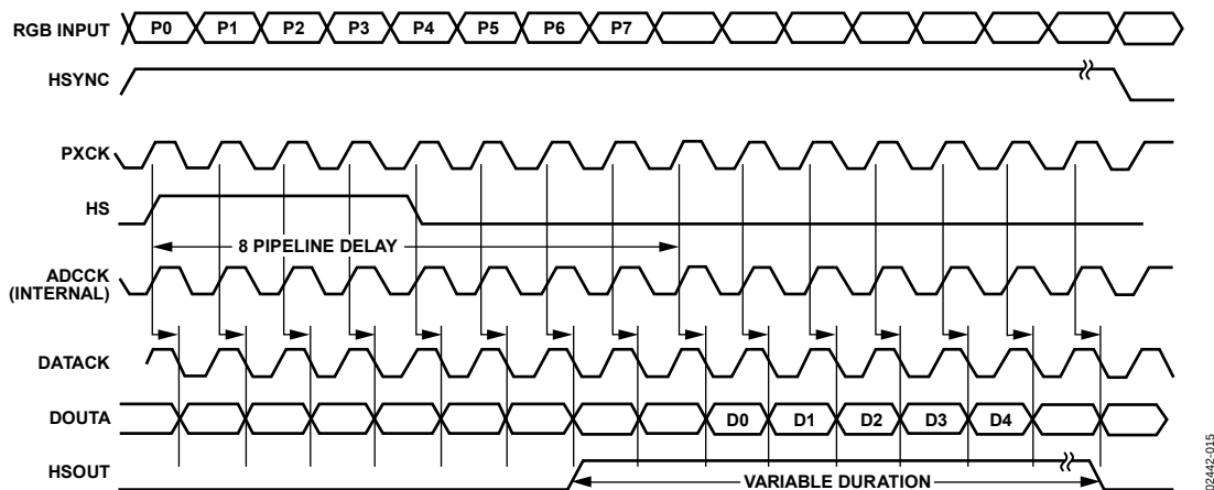
Figure 16. Single-Port Mode
