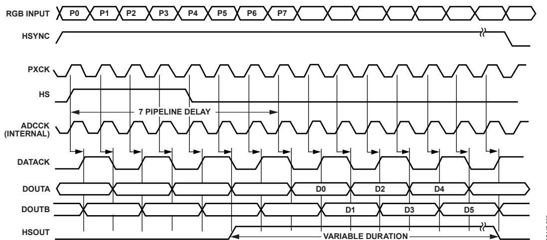
Figure 19. Dual-Port Mode, Interleaved Outputs
