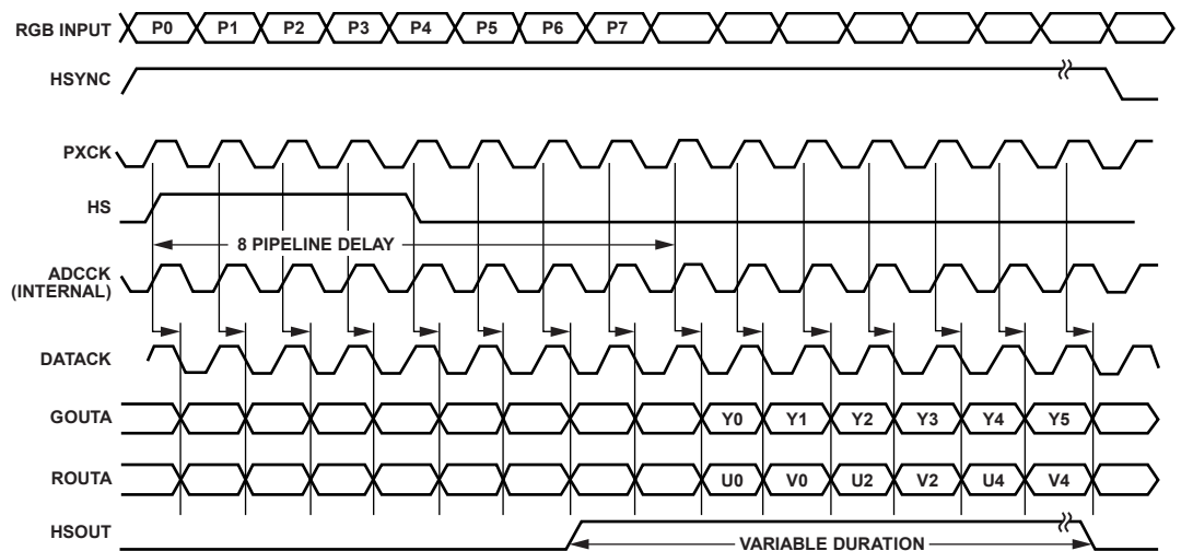
Figure 25. 4:2:2 Output Mode
