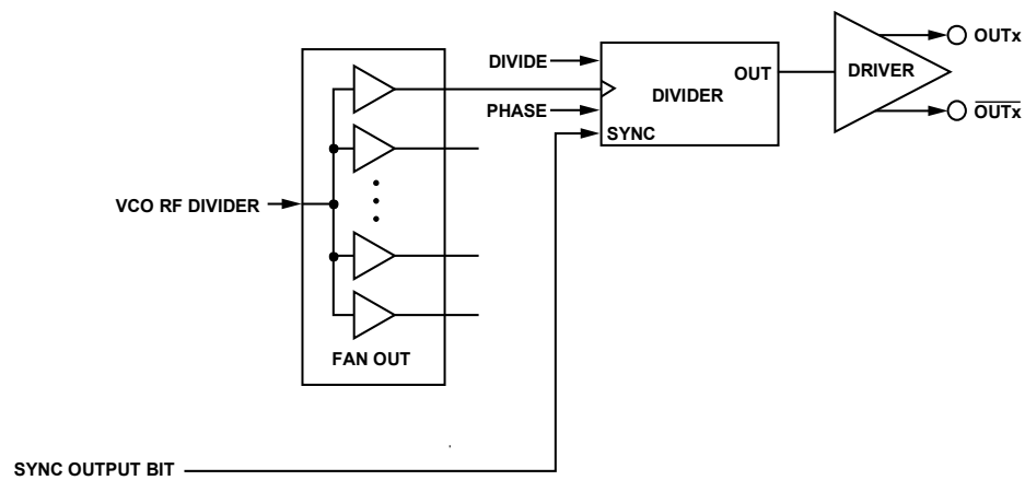
Figure 35. Clock Distribution Synchronization Block Diagram
