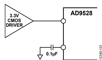
Figure 25. REFx, VCXO Input, Single-Ended Mode Receiver
