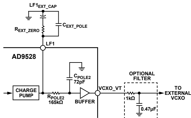
Figure 28. PLL1 Loop Filter
