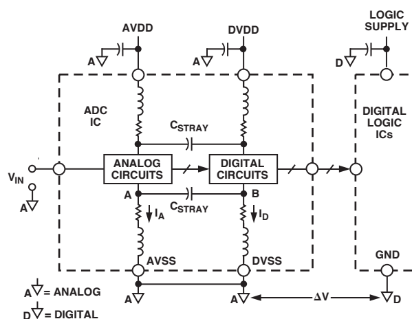
Figure 31. Ground and Power Consideration
