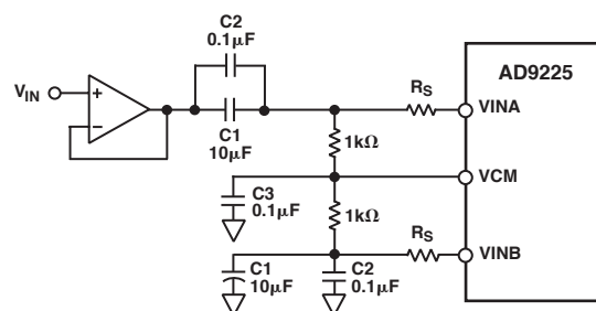
Figure 11. AC-Coupled Input-Flexible Input Span, V_{CM} = 2.5\text{ V}
