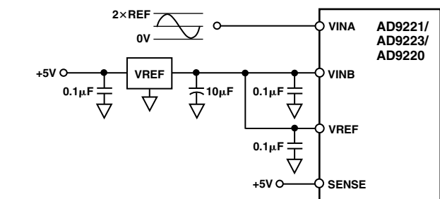
Figure 25. Input Range = 0\text{ V to }2 \times V_{REF}
