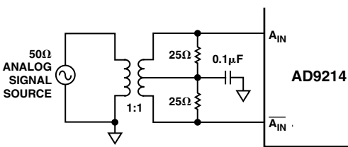
Figure 8. Single-Ended-to-Differential Conversion Using a Transformer
