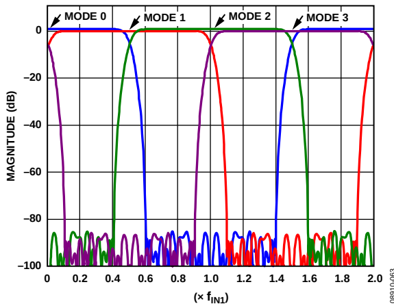
Figure 64. HB1 Filter Modes
