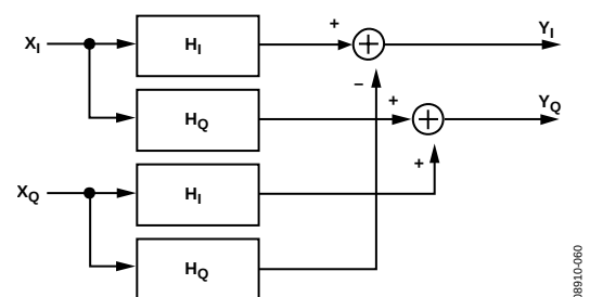
Figure 61. Complex Filter Implementation
