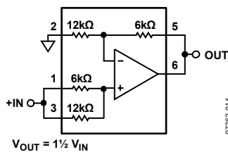
Figure 46. Noninverting Amplifier, G = 1.5
