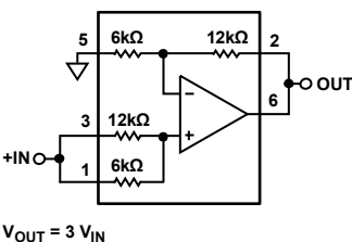
Figure 47. Noninverting Amplifier, G = 3
