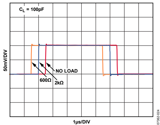
Figure 19. Small-Signal Step Response, Gain = 2
