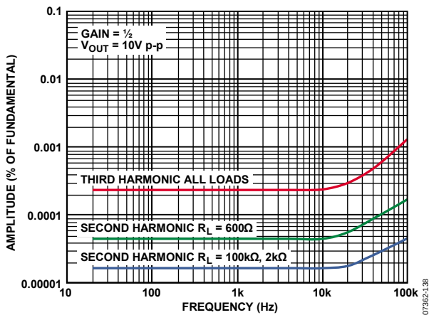
Figure 36. Harmonic Distortion Products vs. Frequency, G = \frac{1}{2}
