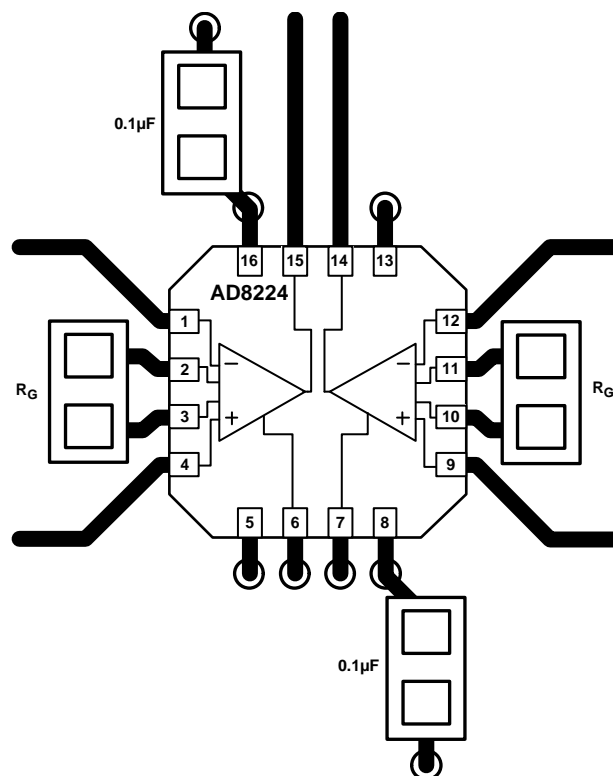
Figure 59. Example Layout
