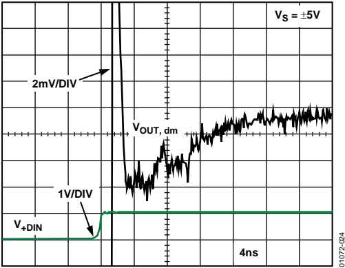
Figure 25. 0.1% Settling Time
