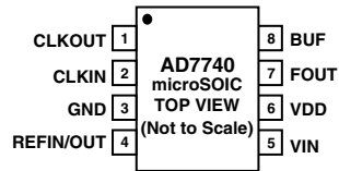
8-Lead MSOP
