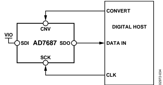
Figure 34. \overline{\text{CS}} Mode, 3-Wire Without BUSY Indicator Connection Diagram (SDI High)
