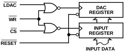
Figure 3. Input Control Logic
