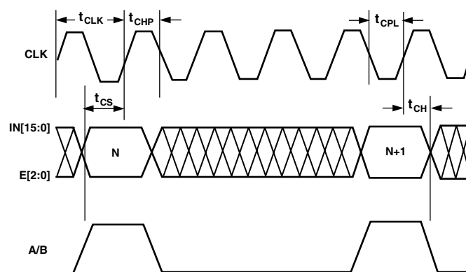
Figure 7. SYNC Master Delay
