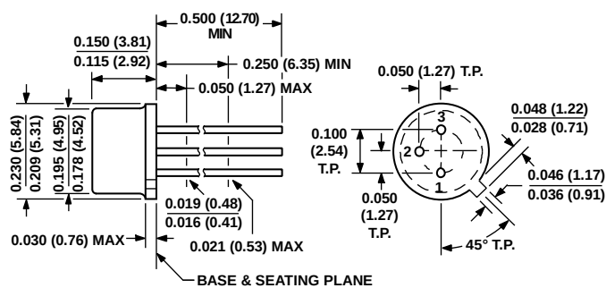
Figure 26. 3-Pin Metal Header Package [TO-52] (H-03-1)
