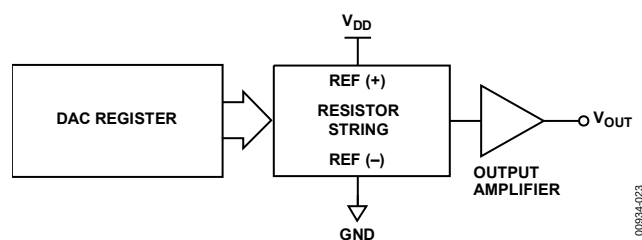
Figure 23. DAC Architecture
