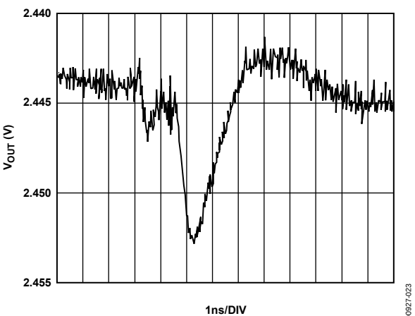
Figure 23. Digital Feedthrough
