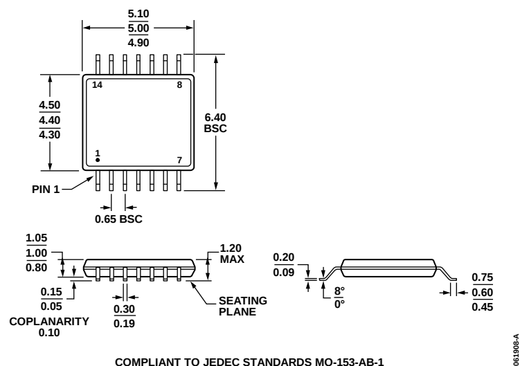
Figure 57. 14-Lead Thin Shrink Small Outline Package [TSSOP] (RU-14) Dimensions shown in millimeters
